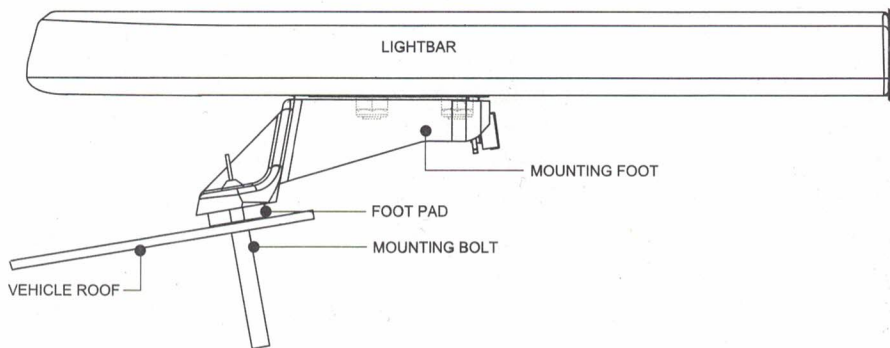
Front view of lightbar with Permanent mount
